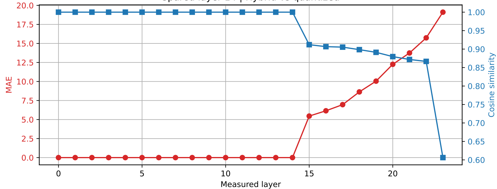
SmolLM2-1.7B-Instruct | Prompt 2 Spared layer 14 | Hybrid vs quantized
