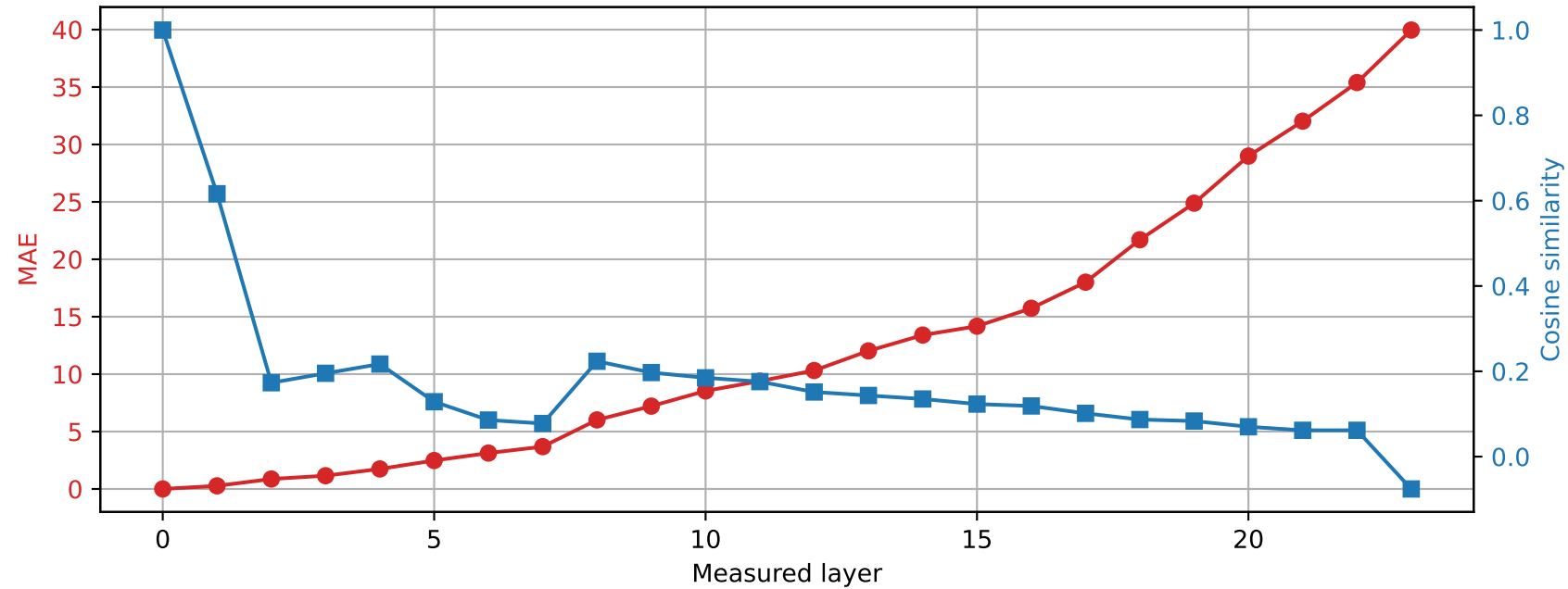
SmolLM2-1.7B-Instruct | Prompt 2 Spared layer 18 | Hybrid vs unquantized
