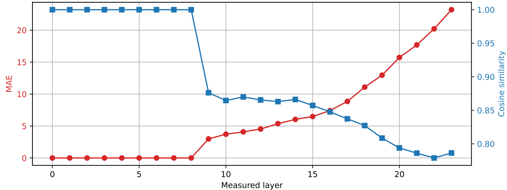
SmolLM2-1.7B-Instruct | Prompt 3 Spared layer 8 | Hybrid vs quantized
