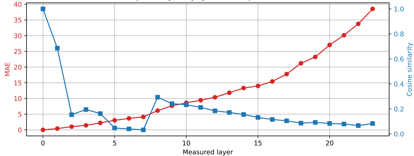
SmolLM2-1.7B-Instruct | Prompt 3 Spared layer 8 | Hybrid vs unquantized
