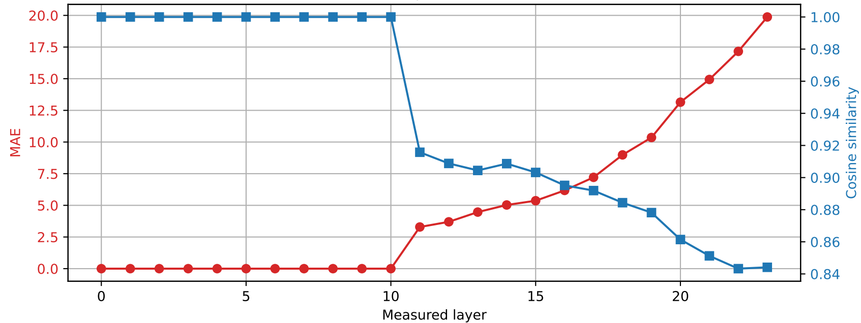
SmolLM2-1.7B-Instruct | Prompt 3 Spared layer 10 | Hybrid vs quantized
