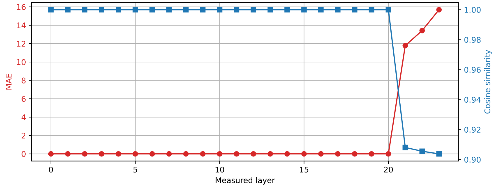
SmolLM2-1.7B-Instruct | Prompt 3 Spared layer 20 | Hybrid vs quantized
