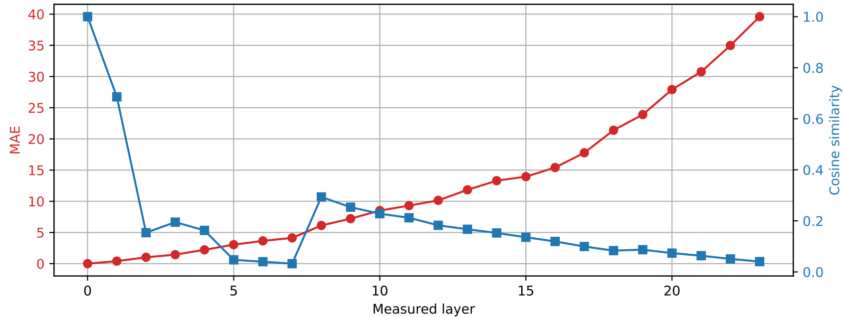
SmolLM2-1.7B-Instruct | Prompt 3 Spared layer 21 | Hybrid vs unquantized
