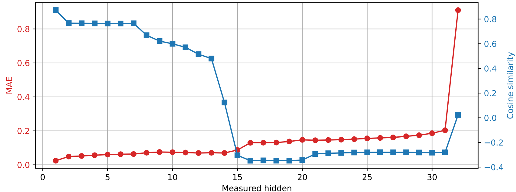
OLMo-7B-hf | Prompt 4 Spared layer 4 | Unquantized vs hybrid
