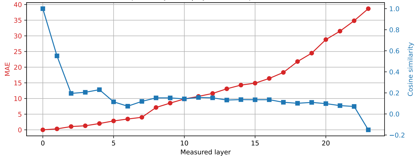
SmolLM2-1.7B-Instruct | Prompt 4 Spared layer 10 | Hybrid vs unquantized
