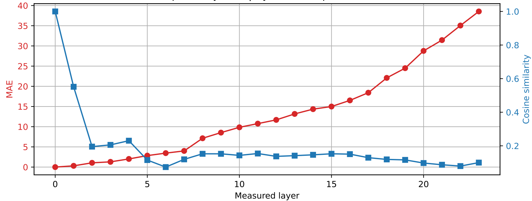
SmolLM2-1.7B-Instruct | Prompt 4 Spared layer 19 | Hybrid vs unquantized
