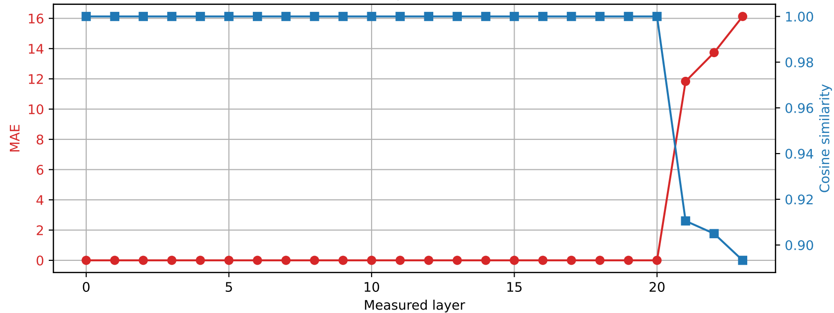
SmolLM2-1.7B-Instruct | Prompt 4 Spared layer 20 | Hybrid vs quantized
