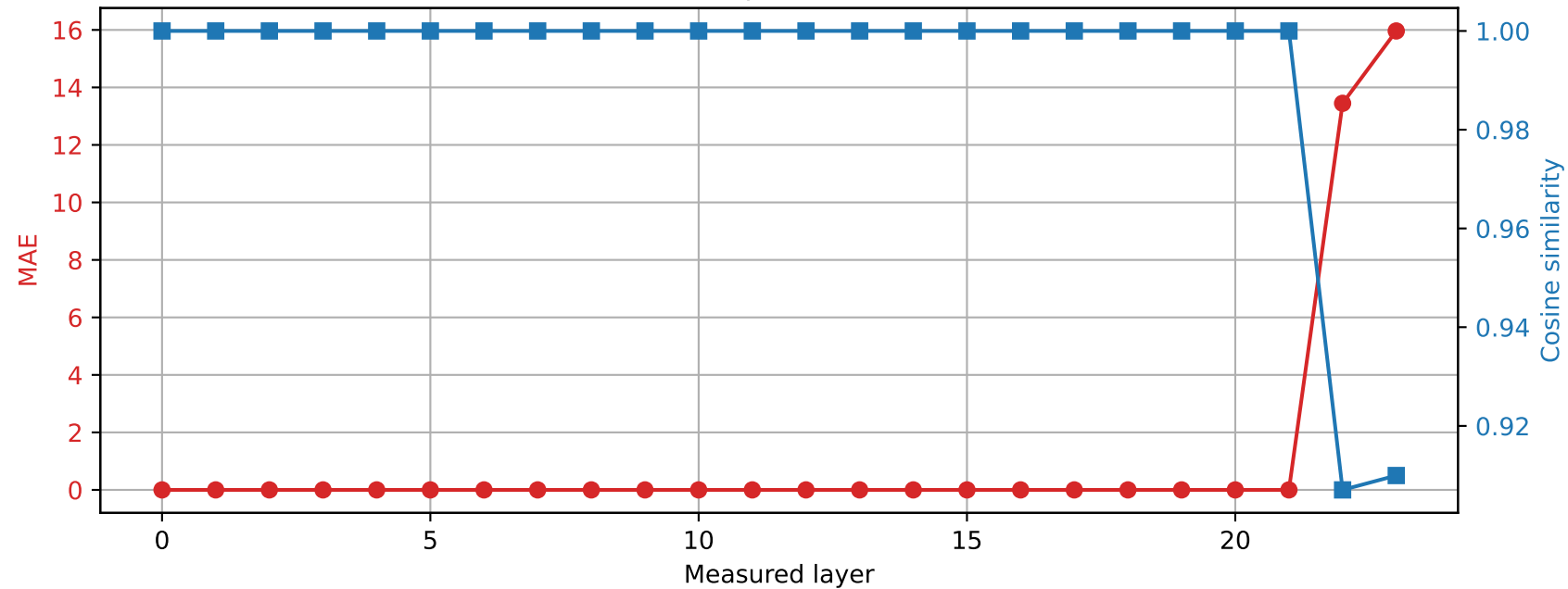
SmolLM2-1.7B-Instruct | Prompt 4 Spared layer 21 | Hybrid vs quantized
