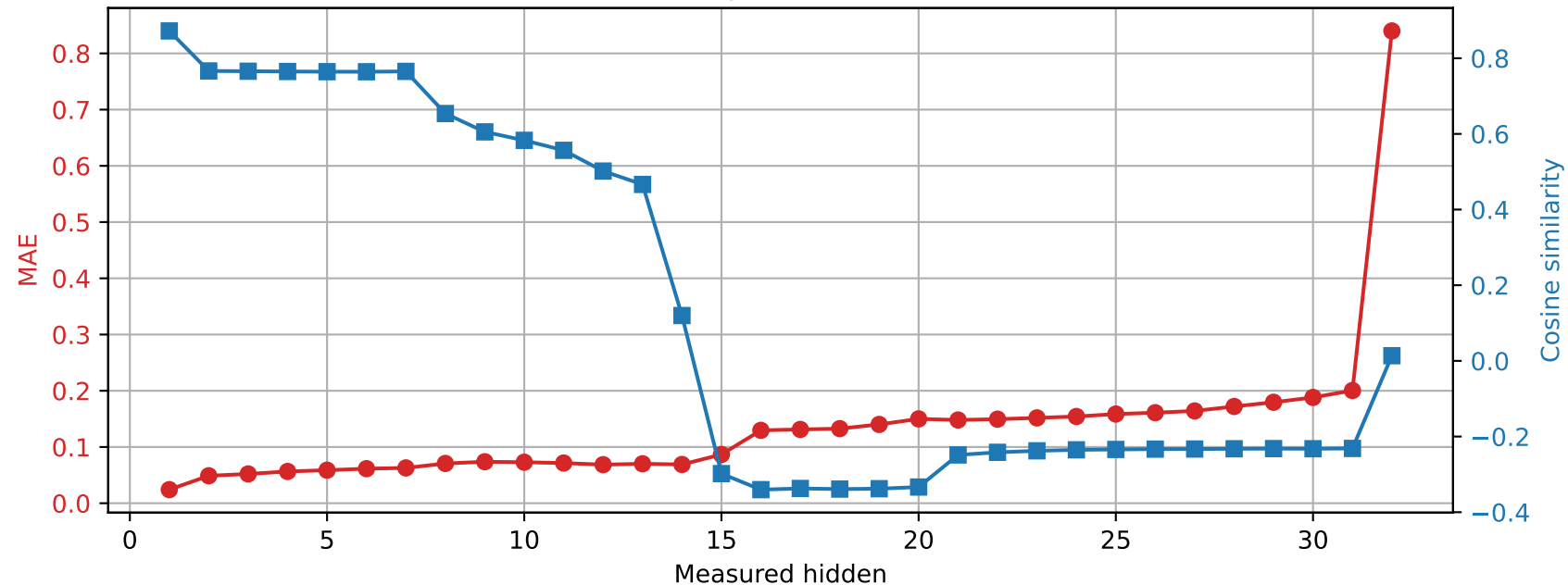
OLMo-7B-hf | Prompt 4 Spared layer 25 | Unquantized vs hybrid
