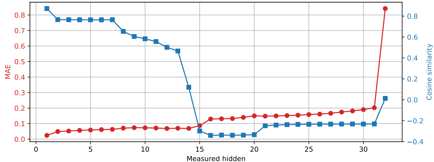
OLMo-7B-hf | Prompt 4 Spared layer 26 | Unquantized vs hybrid
