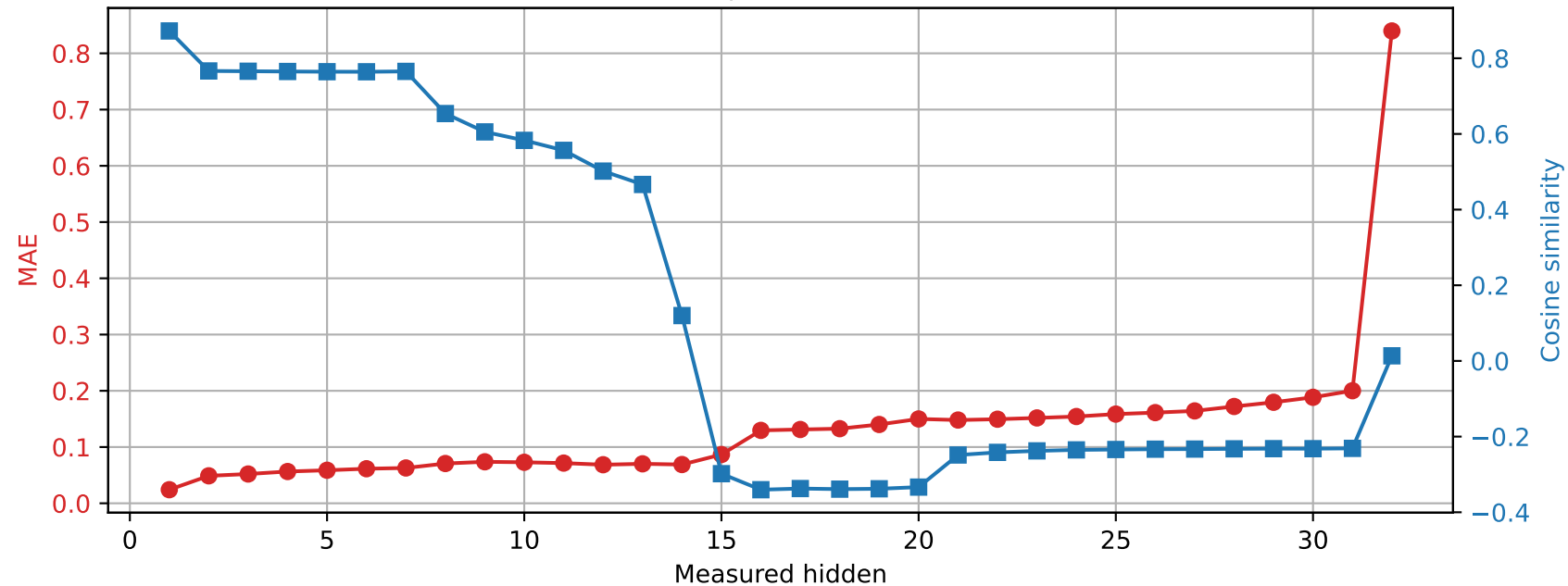
OLMo-7B-hf | Prompt 4 Spared layer 29 | Unquantized vs hybrid
