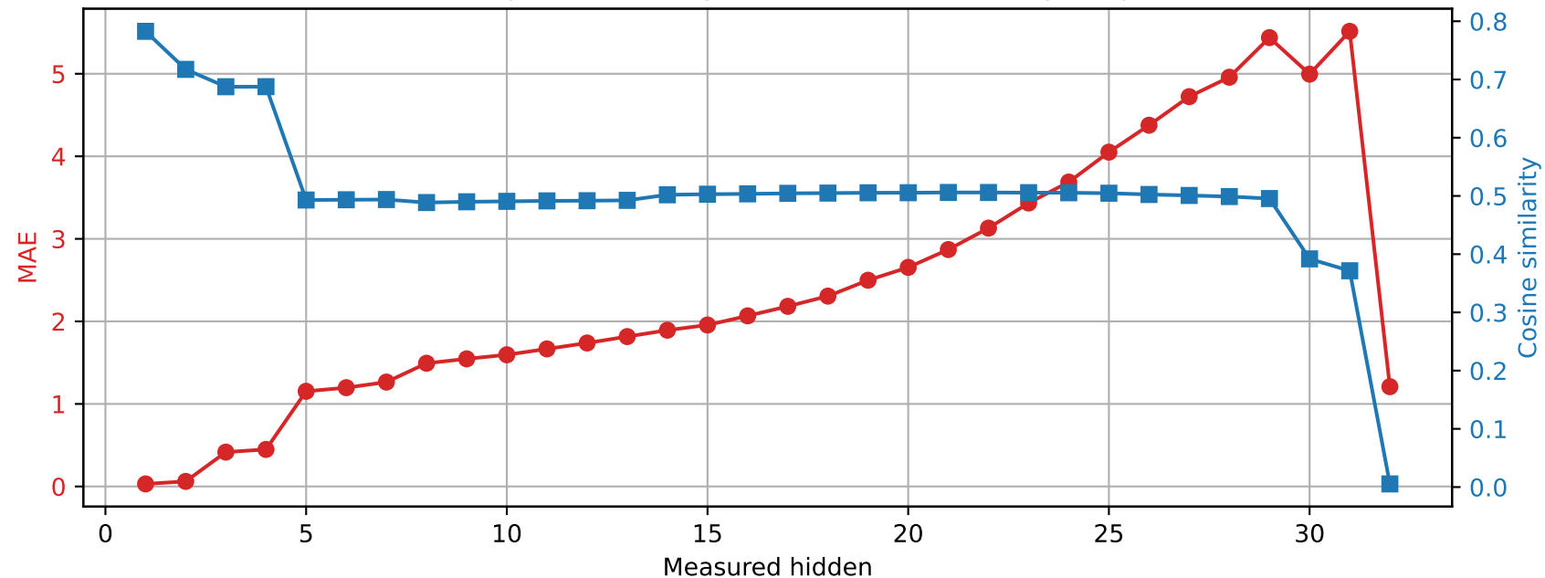
Phi-3-mini-4k-instruct Mean unquantized vs quantized int4 across 5 prompts
