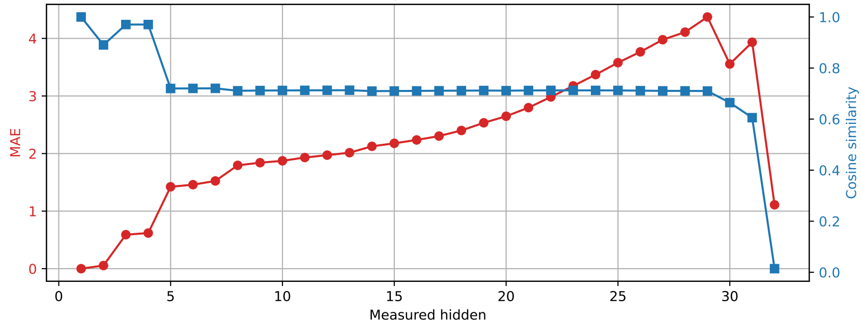
Phi-3-mini-4k-instruct | Prompt 0 Spared layer 0 | Unquantized vs hybrid
