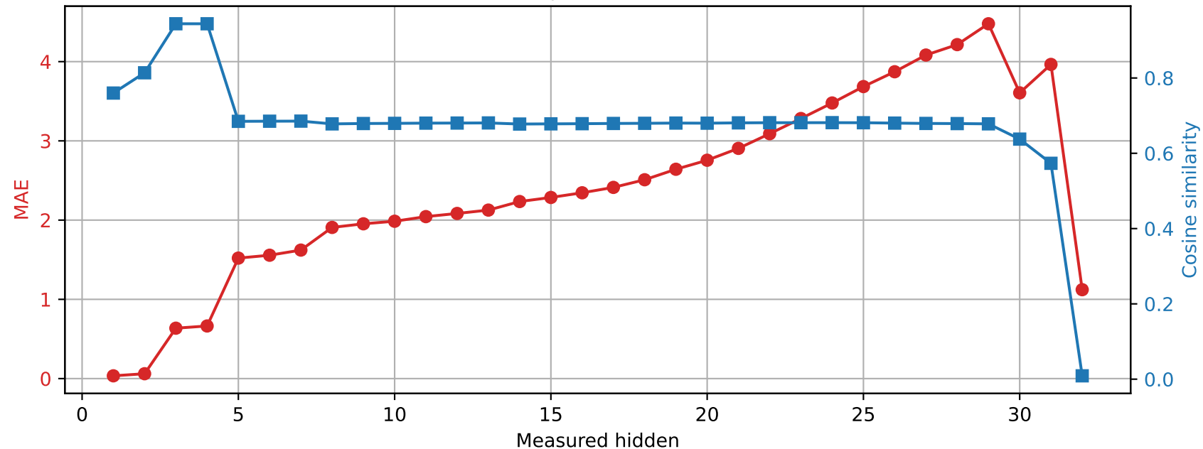
Phi-3-mini-4k-instruct | Prompt 0 Spared layer 1 | Unquantized vs hybrid
