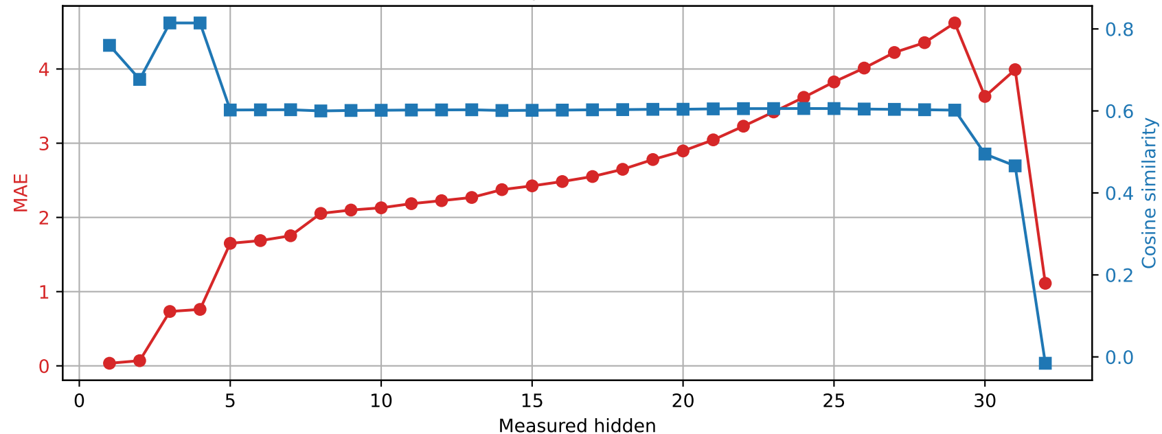
Phi-3-mini-4k-instruct | Prompt 0 Spared layer 6 | Unquantized vs hybrid
