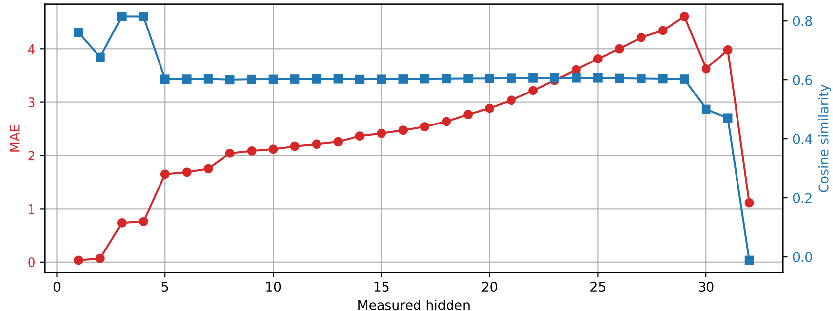
Phi-3-mini-4k-instruct | Prompt 0 Spared layer 10 | Unquantized vs hybrid
