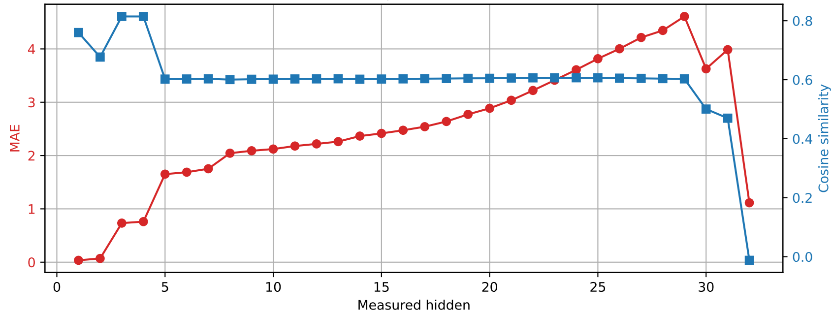
Phi-3-mini-4k-instruct | Prompt 0 Spared layer 11 | Unquantized vs hybrid
