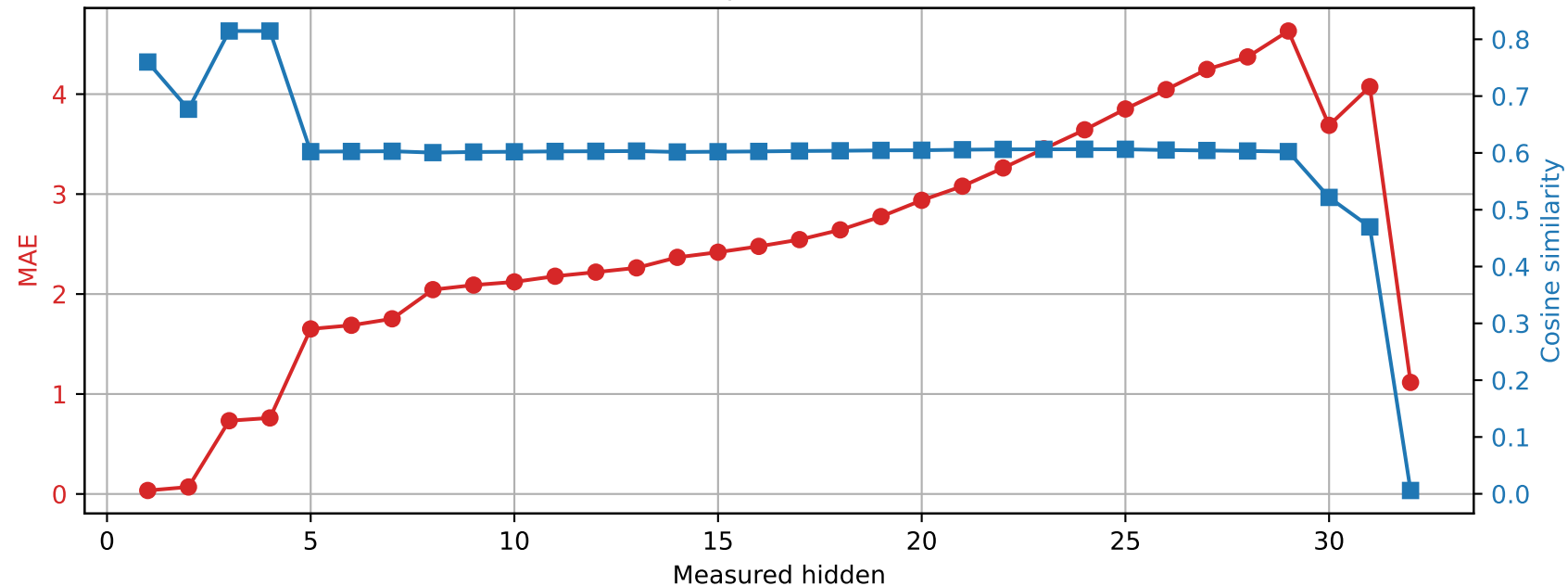
Phi-3-mini-4k-instruct | Prompt 0 Spared layer 19 | Unquantized vs hybrid
