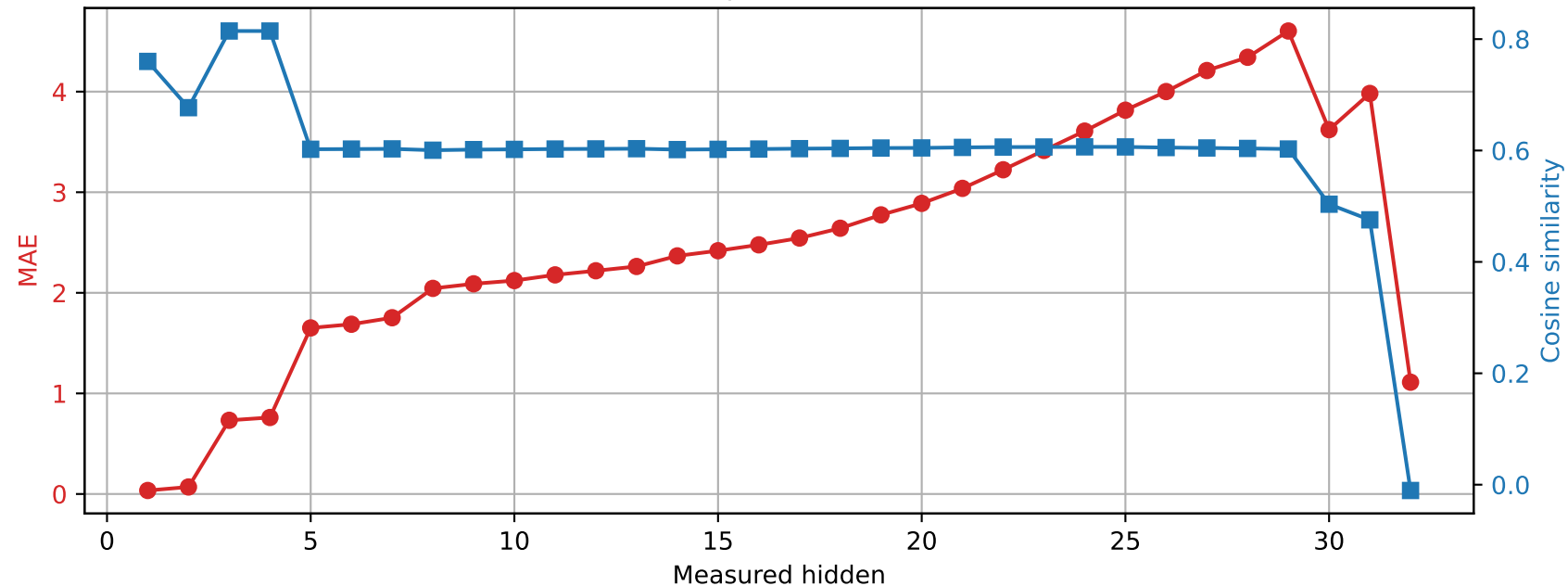
Phi-3-mini-4k-instruct | Prompt 0 Spared layer 23 | Unquantized vs hybrid
