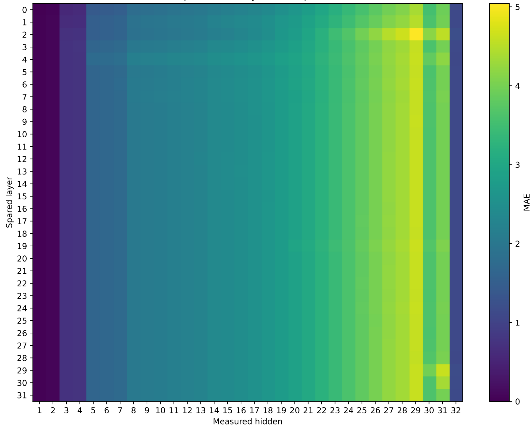
Phi-3-mini-4k-instruct | Prompt 0 Unquantized vs hybrid MAE | int4
