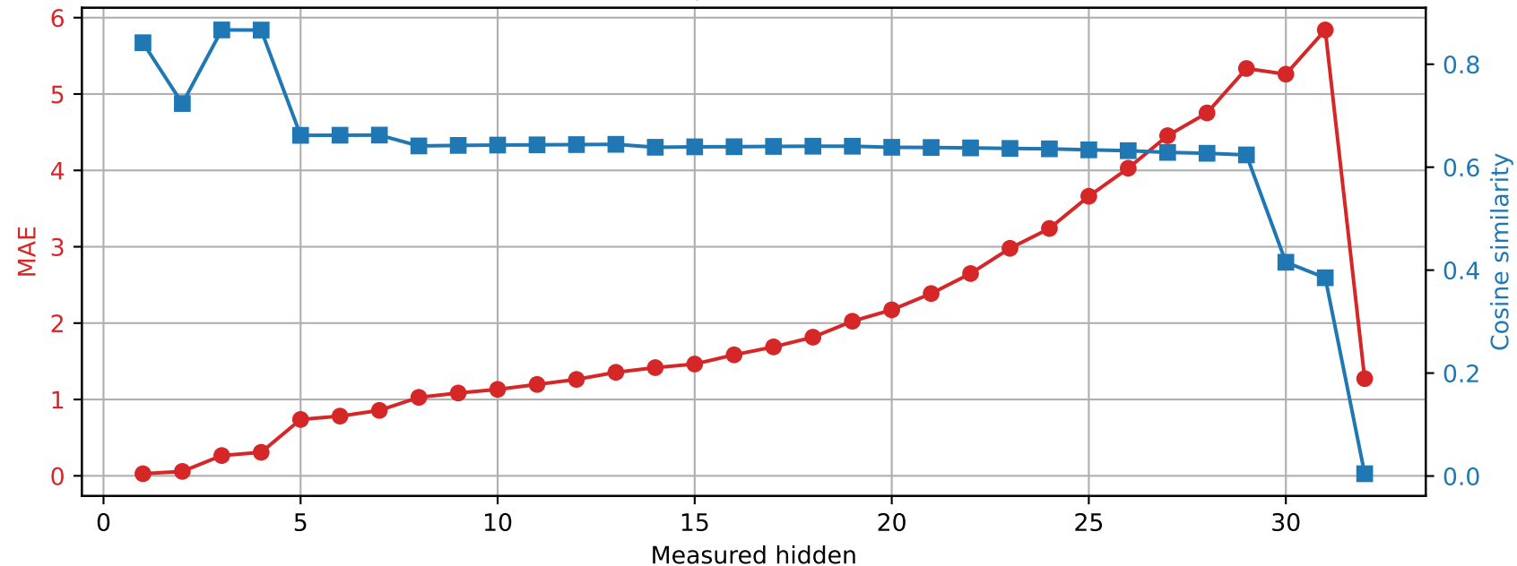
Phi-3-mini-4k-instruct | Prompt 1 Spared layer 3 | Unquantized vs hybrid
