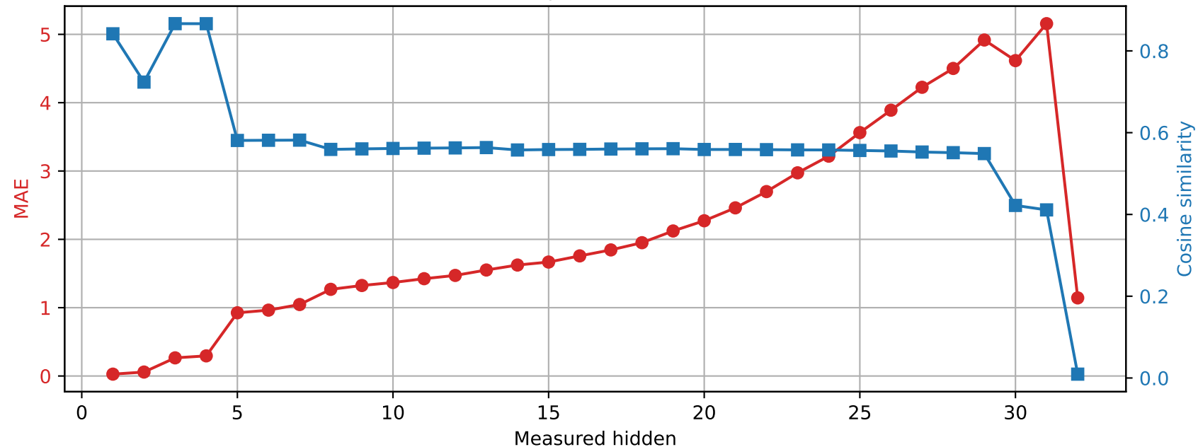
Phi-3-mini-4k-instruct | Prompt 1 Spared layer 6 | Unquantized vs hybrid
