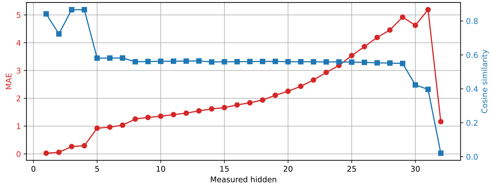
Phi-3-mini-4k-instruct | Prompt 1 Spared layer 16 | Unquantized vs hybrid
