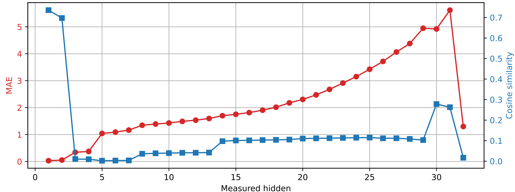
Phi-3-mini-4k-instruct | Prompt 2 Spared layer 2 | Unquantized vs hybrid
