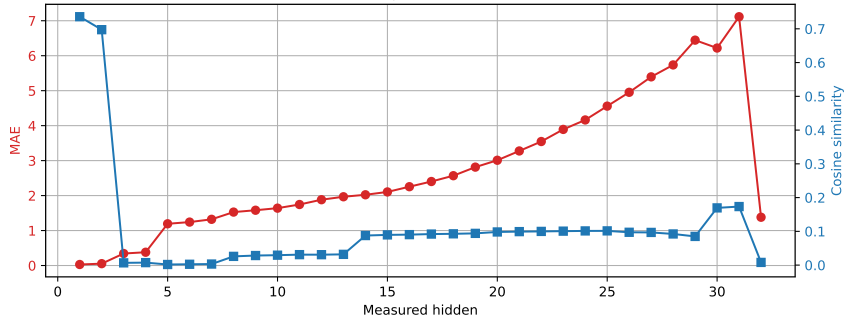
Phi-3-mini-4k-instruct | Prompt 2 Spared layer 11 | Unquantized vs hybrid
