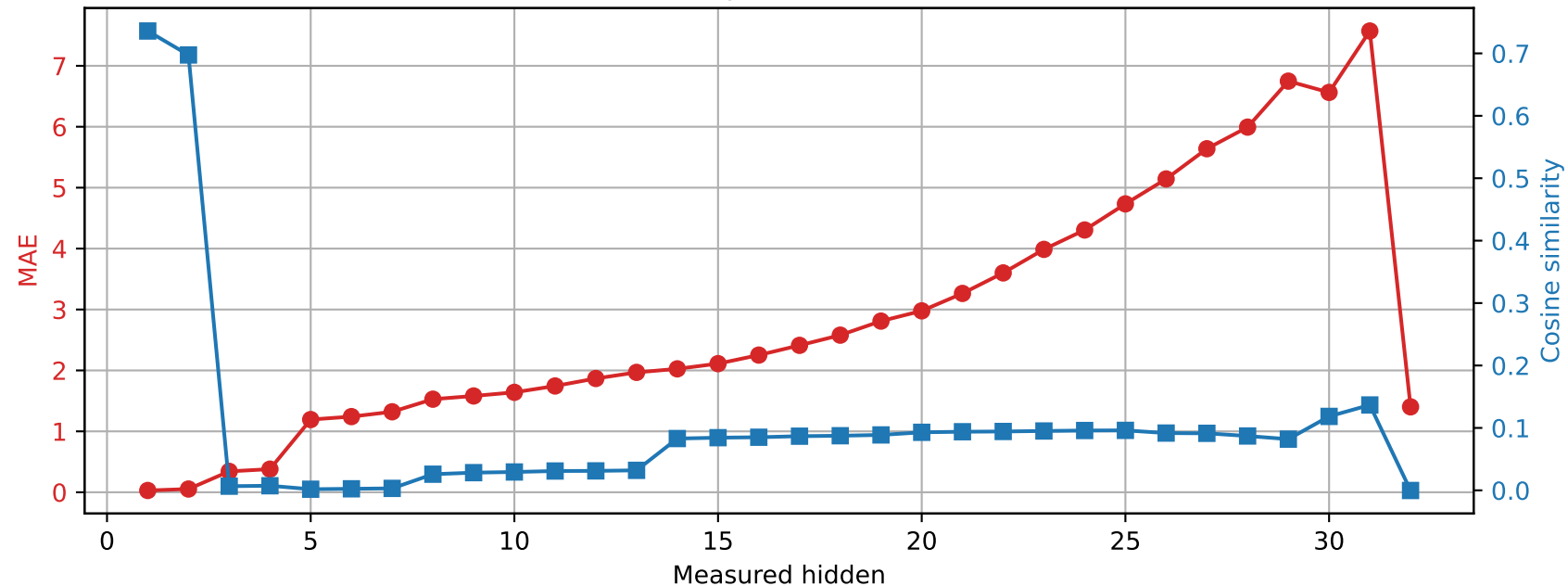
Phi-3-mini-4k-instruct | Prompt 2 Spared layer 12 | Unquantized vs hybrid
