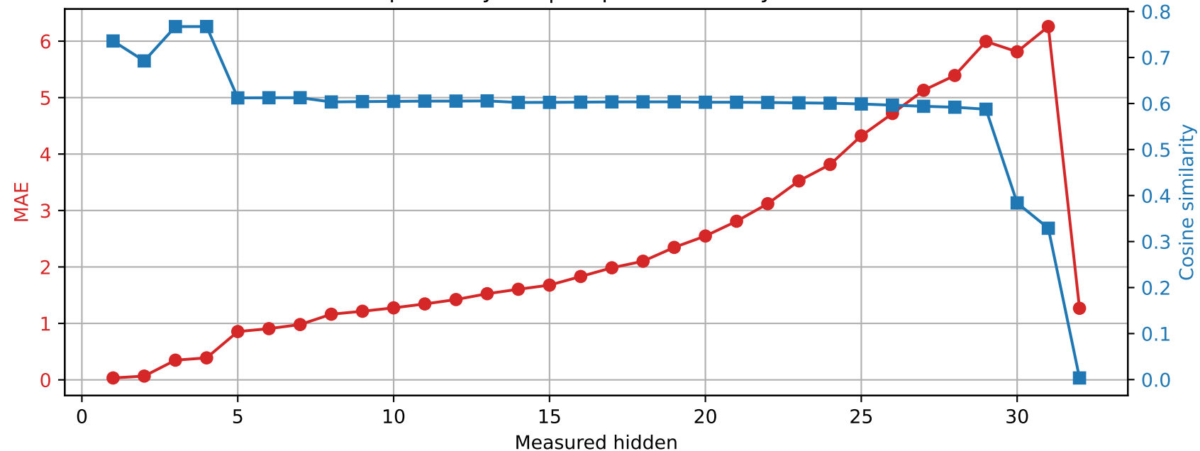
Phi-3-mini-4k-instruct | Prompt 3 Spared layer 6 | Unquantized vs hybrid
