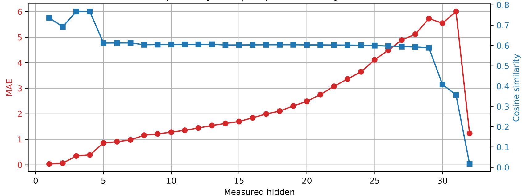
Phi-3-mini-4k-instruct | Prompt 3 Spared layer 22 | Unquantized vs hybrid
