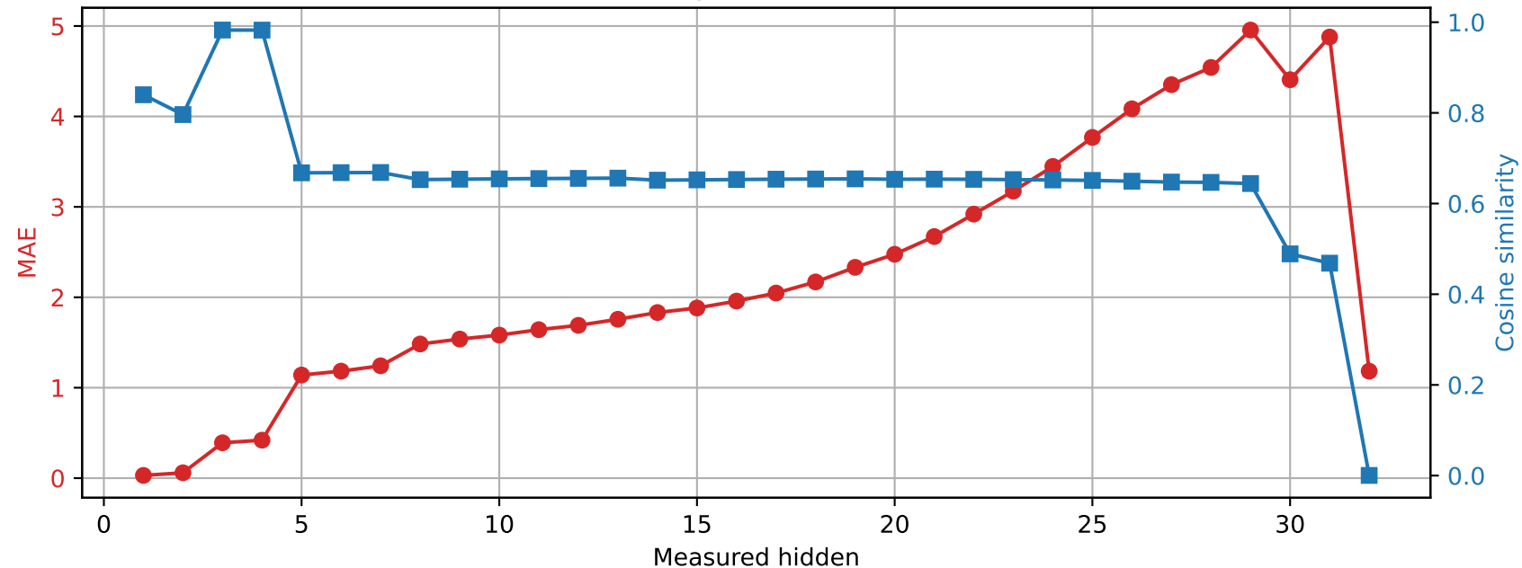
Phi-3-mini-4k-instruct | Prompt 4 Spared layer 6 | Unquantized vs hybrid
