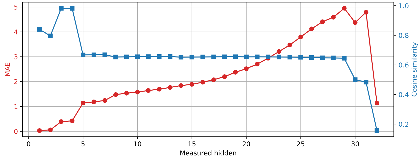
Phi-3-mini-4k-instruct | Prompt 4 Spared layer 31 | Unquantized vs hybrid
