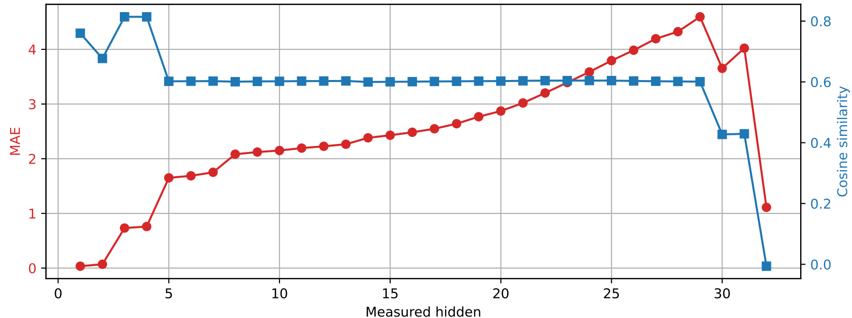
Phi-3-mini-4k-instruct | Prompt 0 Spared layer 7 | Unquantized vs hybrid
