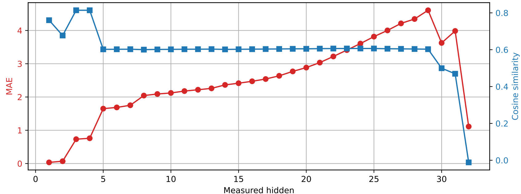
Phi-3-mini-4k-instruct | Prompt 0 Spared layer 8 | Unquantized vs hybrid
