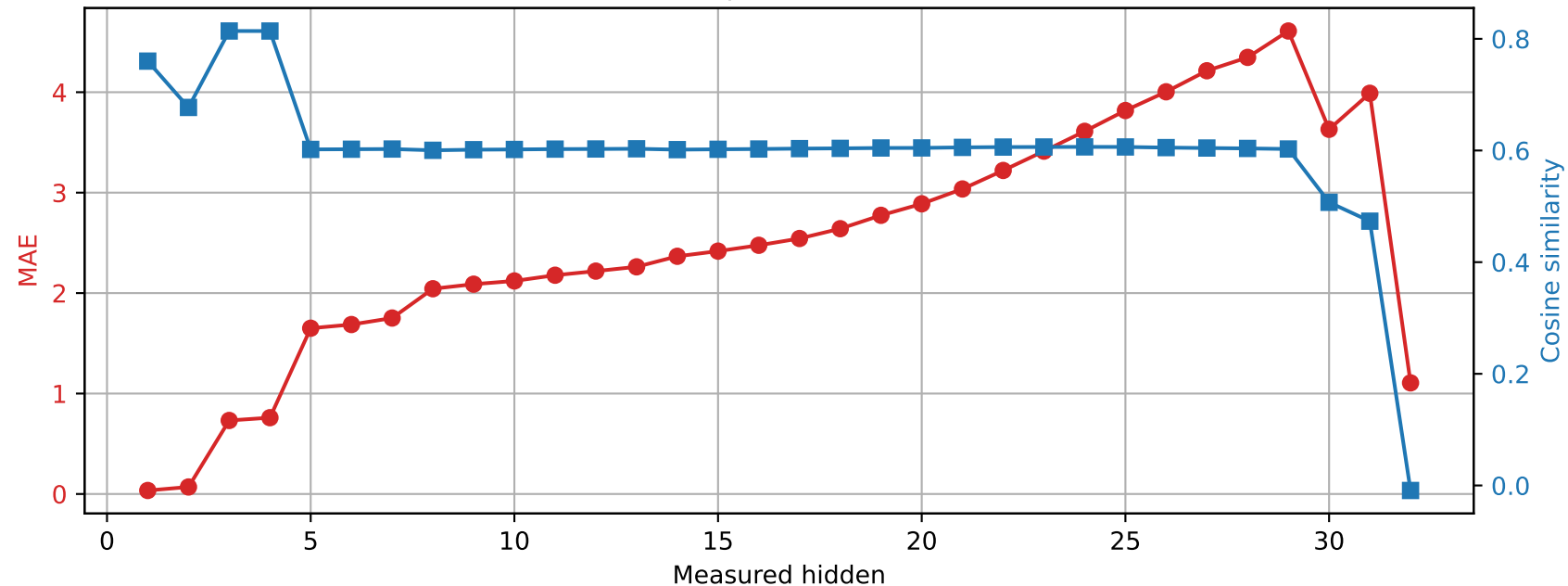
Phi-3-mini-4k-instruct | Prompt 0 Spared layer 20 | Unquantized vs hybrid
