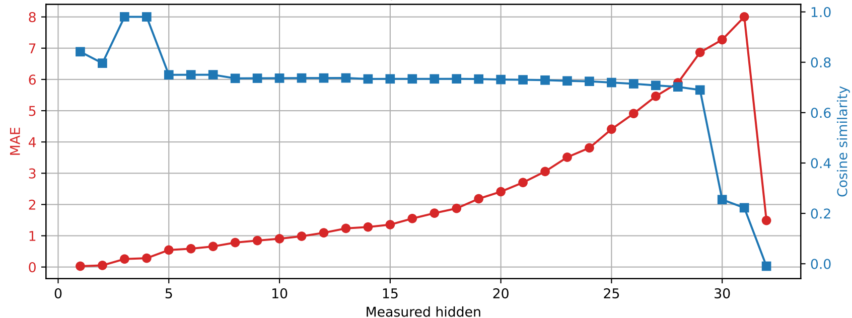
Phi-3-mini-4k-instruct | Prompt 1 Spared layer 1 | Unquantized vs hybrid
