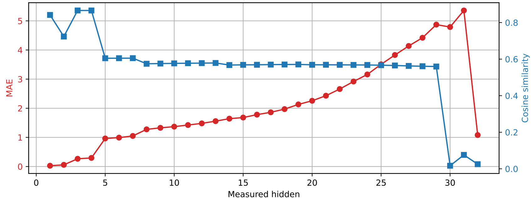
Phi-3-mini-4k-instruct | Prompt 1 Spared layer 4 | Unquantized vs hybrid
