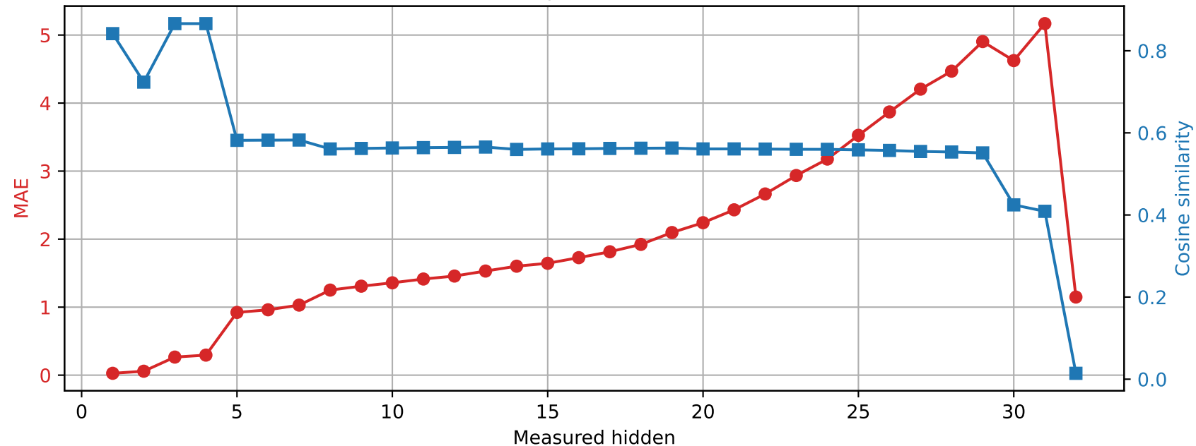
Phi-3-mini-4k-instruct | Prompt 1 Spared layer 9 | Unquantized vs hybrid
