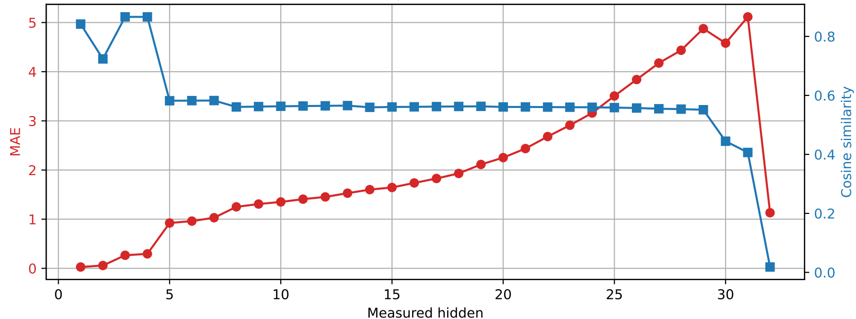
Phi-3-mini-4k-instruct | Prompt 1 Spared layer 22 | Unquantized vs hybrid
