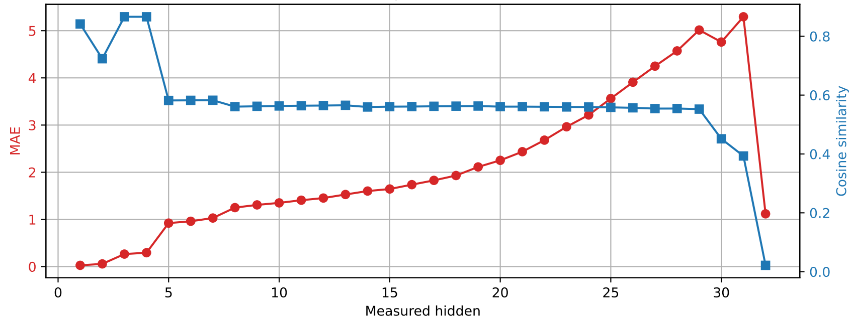
Phi-3-mini-4k-instruct | Prompt 1 Spared layer 27 | Unquantized vs hybrid
