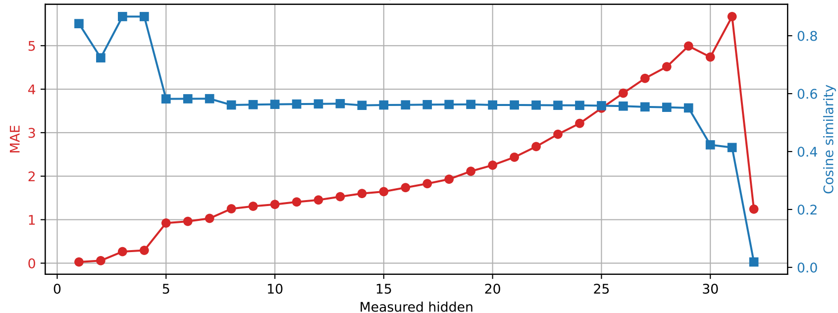
Phi-3-mini-4k-instruct | Prompt 1 Spared layer 30 | Unquantized vs hybrid
