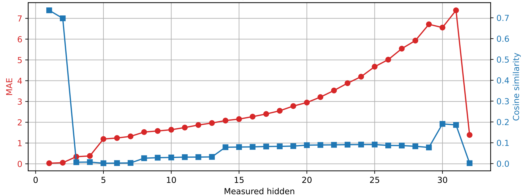
Phi-3-mini-4k-instruct | Prompt 2 Spared layer 13 | Unquantized vs hybrid
