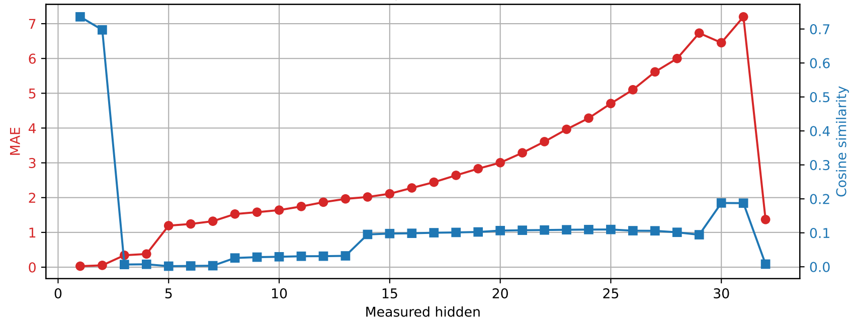
Phi-3-mini-4k-instruct | Prompt 2 Spared layer 17 | Unquantized vs hybrid
