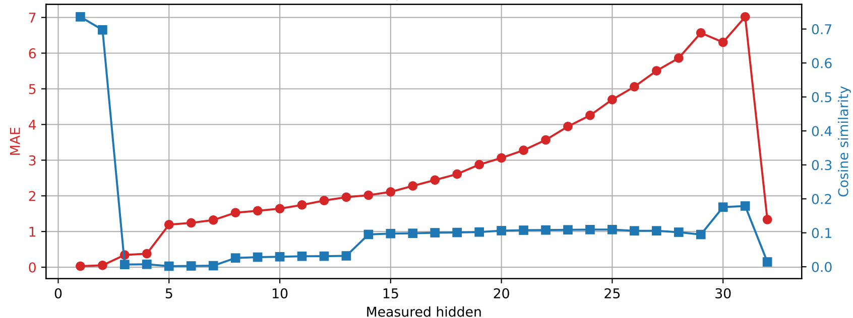
Phi-3-mini-4k-instruct | Prompt 2 Spared layer 20 | Unquantized vs hybrid
