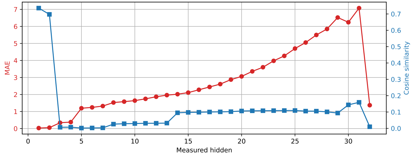
Phi-3-mini-4k-instruct | Prompt 2 Spared layer 21 | Unquantized vs hybrid
