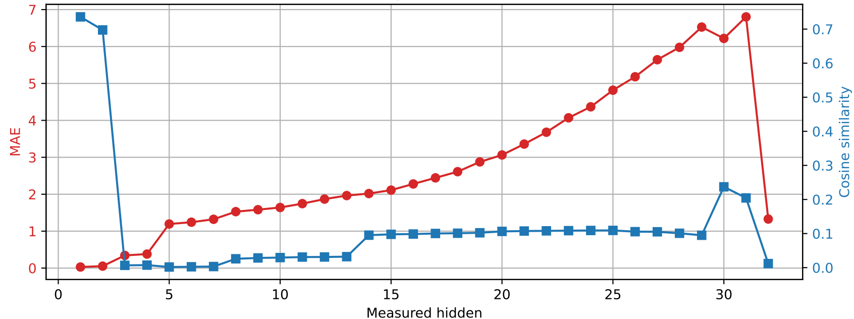
Phi-3-mini-4k-instruct | Prompt 2 Spared layer 28 | Unquantized vs hybrid
