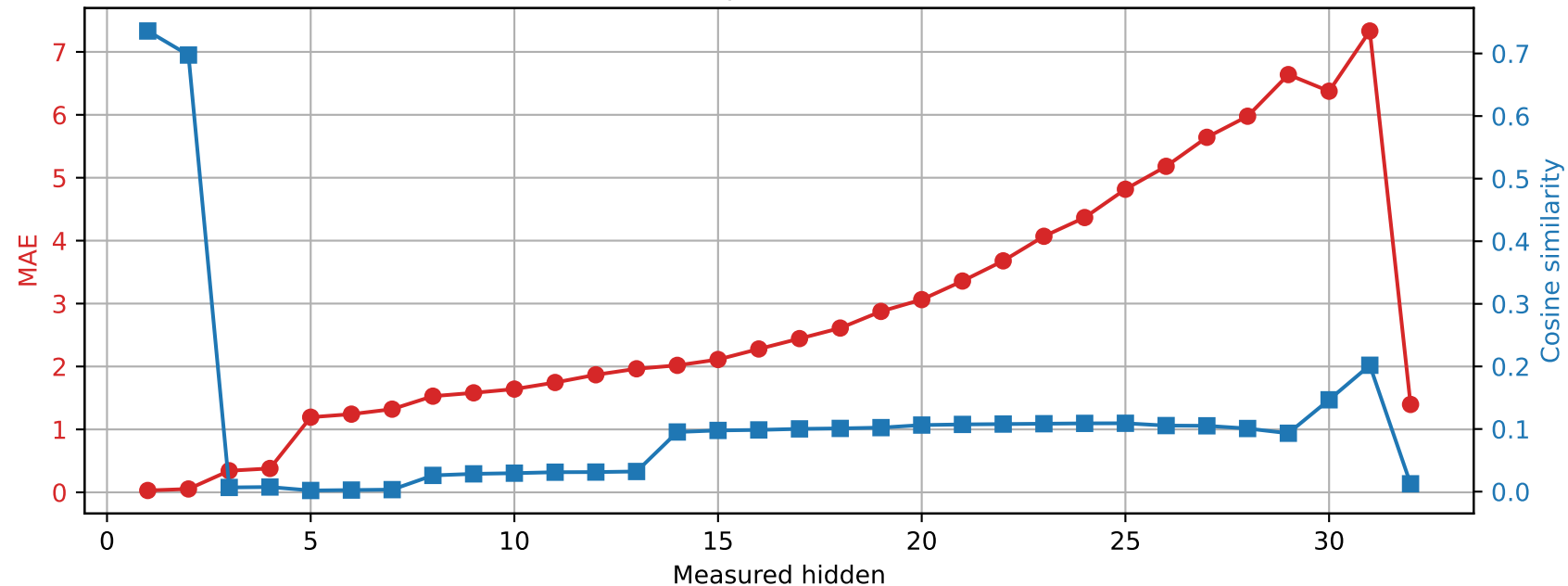
Phi-3-mini-4k-instruct | Prompt 2 Spared layer 30 | Unquantized vs hybrid
