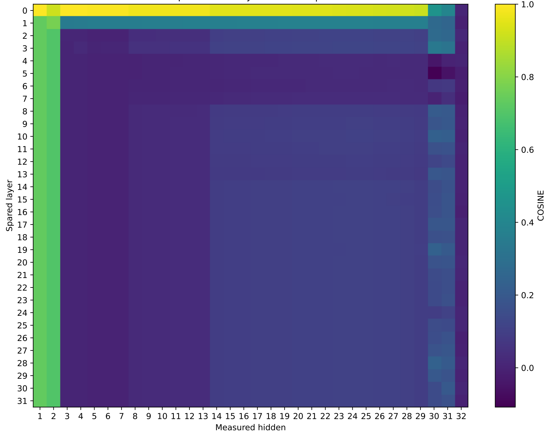
Phi-3-mini-4k-instruct | Prompt 2 Unquantized vs hybrid cos sim | int4
